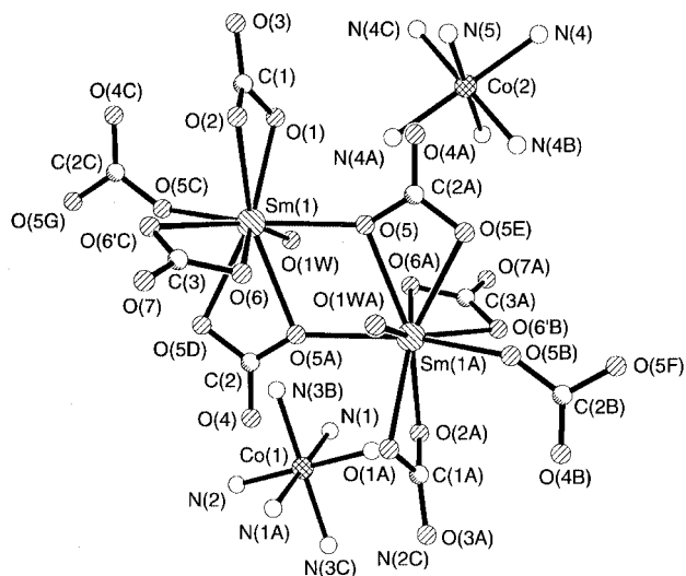
Fig. 1 Ball-and-stick view of two [\text{Sm}(\text{CO}_3)_3(\text{H}_2\text{O})]^{3-} moieties also showing the location of the [\text{Co}(\text{NH}_3)_6]^{3+} cations within the lattice. Selected bond lengths and angles: Sm(1)–O(1) 2.444(7), Sm(1)–O(2) 2.442(9), Sm(1)–O(5) 2.391(5), Sm(1)–O(5)#2 2.516(5), Sm(1)–O(6) 2.457(14), Sm(1)–O(6')#1 2.516(9), Sm(1)–O(1W) 2.568(6); O(1)–Sm(1)–O(2) 53.5(3), O(1)–Sm(1)–O(5) 80.98(13), O(1)–Sm(1)–O(6) 135.2(4), O(1)–Sm(1)–O(1W) 74.1(2), O(2)–Sm(1)–O(5) 94.42(14), O(6)–Sm(1)–O(6')#1 52.3(5), O(5)#2–Sm(1)–O(1W) 75.2(2), O(5)#3–Sm(1)–O(6) 69.0(4), O(5)#3–Sm(1)–O(6')#1 105.6(3), O(5)#3–Sm(1)–O(1W) 75.2(2), O(2)–Sm(1)–O(6) 84.6(4), O(2)–Sm(1)–O(6')#1 69.5(3), O(5)–Sm(1)–O(6) 88.1(4), O(5)–Sm(1)–O(5)#3 66.84(19), O(5)–Sm(1)–O(1W) 75.72(15), O(5)#1–Sm(1)–O(6')#1 73.0(3), O(5)#2–Sm(1)–O(5)#3 50.5(2), O(5)#2–Sm(1)–O(6) 83.7(4), O(5)#2–Sm(1)–O(6')#1 79.3(3), Sm(1)–O(5)–Sm(1)#3 113.16(19). Symmetry transformations used to generate equivalent atoms: #1 x, -y + 1, z ; #2 -x + 1/2, y + 1/2, -z + 1 ; #3 -x + 1/2, -y + 1/2, -z + 1 .
